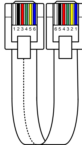
flat cable
