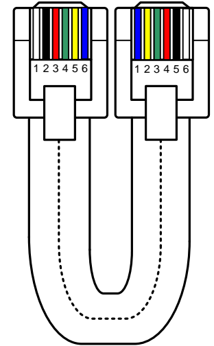
flat cable
