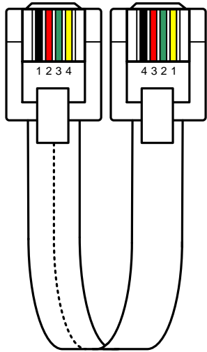
flat cable
