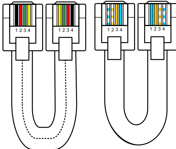
round cable (twisted pair)
