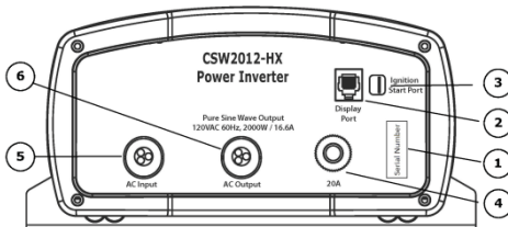
Figure 1-1, Front Panel Features
